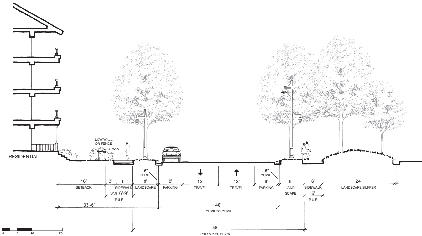
Figure 3.B.22: Kaiser Place Cross Section
